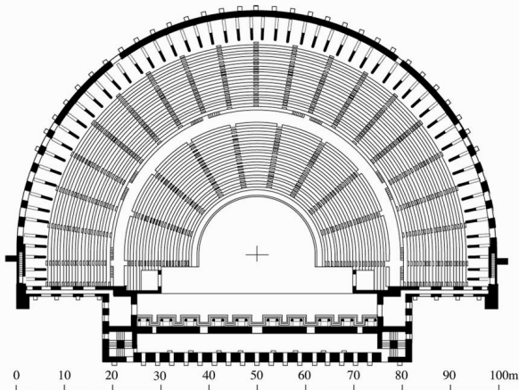
The Roman Theatre at Aspendos (modern Belkiz, Turkey). Cavea width: 95.48 m, orchestra width: 23.87 m; capacity: 15,000; ca. 161-169 AD. Plan (T.H. after Lanckoronski)
